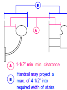
Wall Clearance
