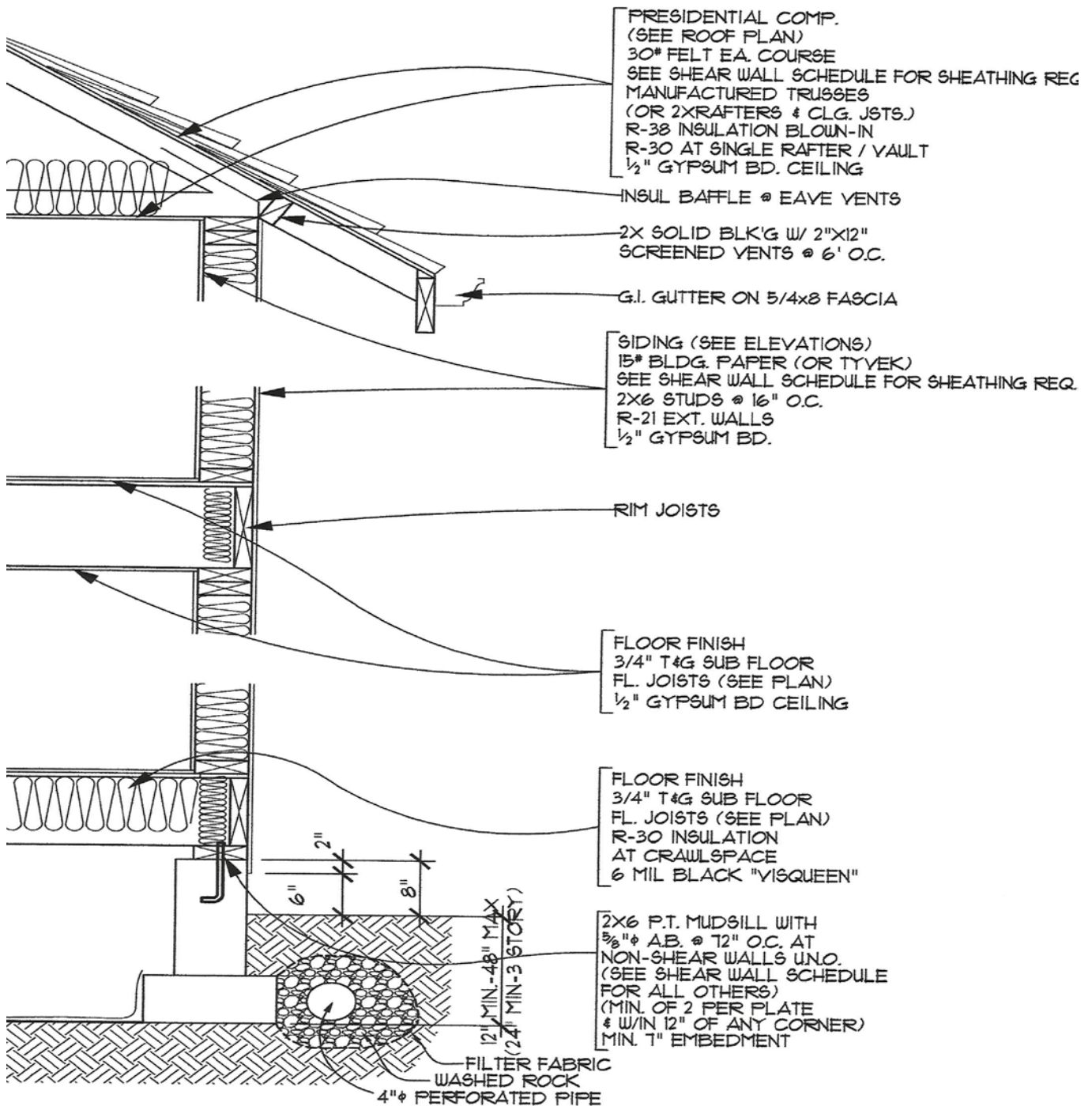
TYPICAL WALL SECTION
